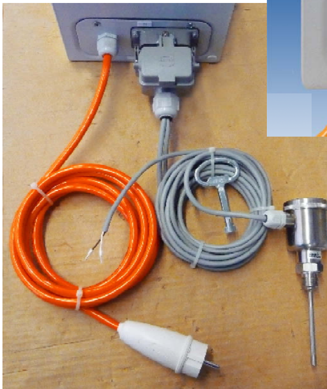
Abb. 3 Anschlüsse
